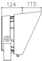
遮光罩/Visor
