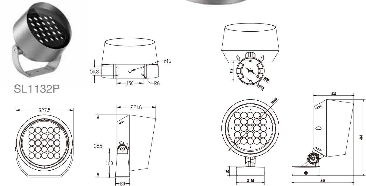
一体压铸 相变液冷 Integrated die casting&phase change liquid cooling
