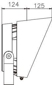
遮光罩/Visor
