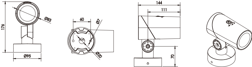
背部角度调节旋钮 Back angle adjustment knob
