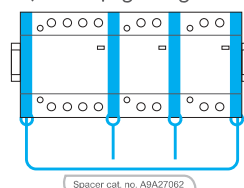
Spacer rail, no. A9A27062
