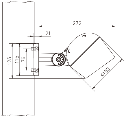
适配树杆尺寸(168–268)mm AVL Dia of pole(168–268)mm
