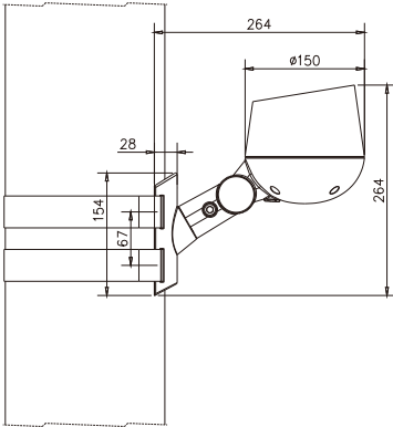
适配杆径(67–325)mm T≥4 AVL Dia of pole(67–325)mm T≥4
